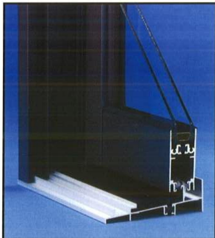
Thermal Barrier frame with optimum 3/8-in. air space
